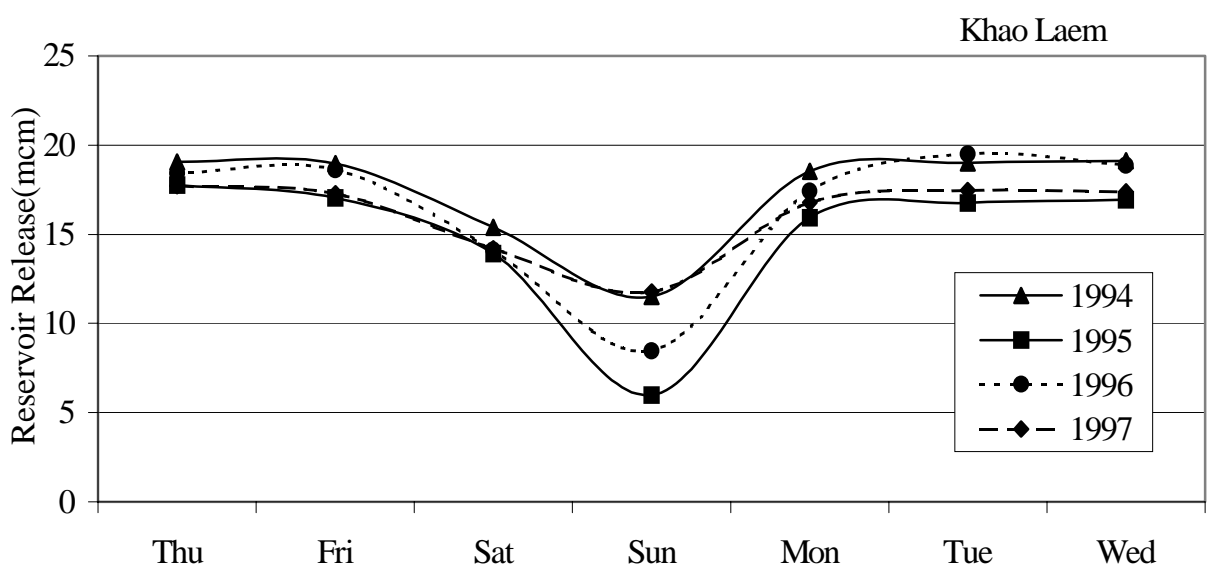
Figure 6 Release Characteristics of Srinagarind, Tha Thung Na and Khao Laem Reservoirs during 1994 - 1997
