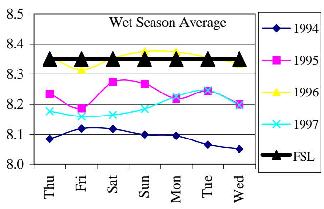
Figure 8 Water Level Characteristics Upstream of The Selected Cross Regulators in Thamaka and Song Phi Nong Irrigation Projects
